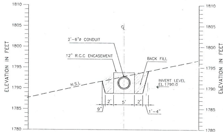
SECTION F-F
