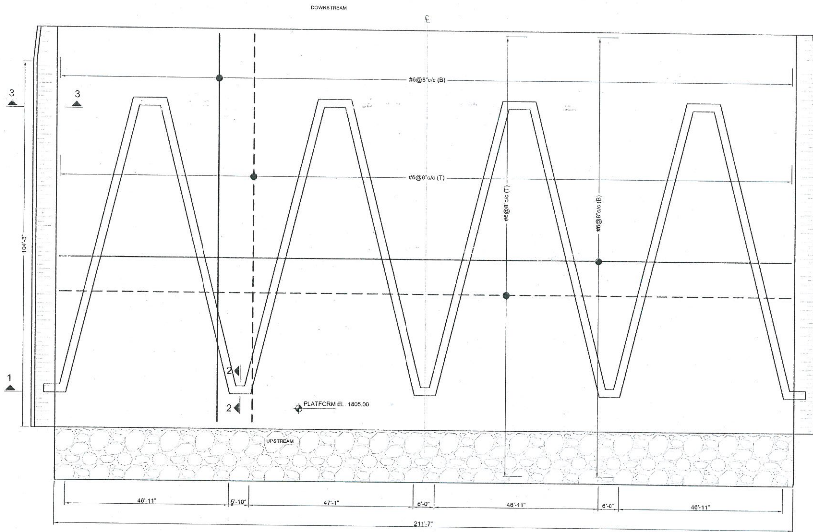
REINFORCEMENT PLAN
