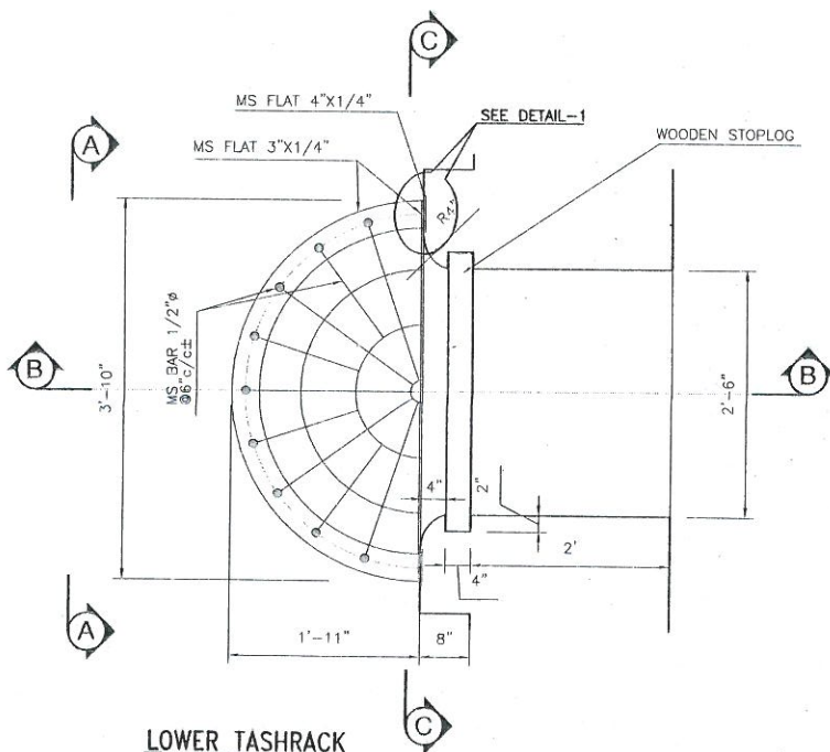
LOWER TASHRACK PLAN
