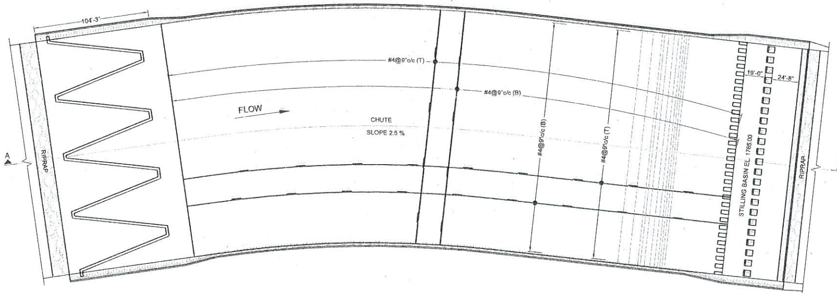
SPILLWAY PLAN
