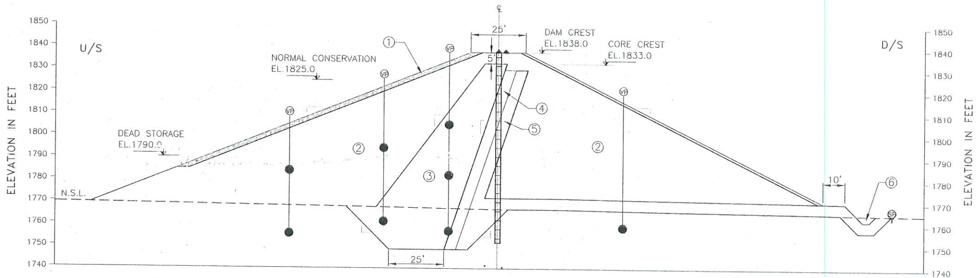
SECTION G-G
