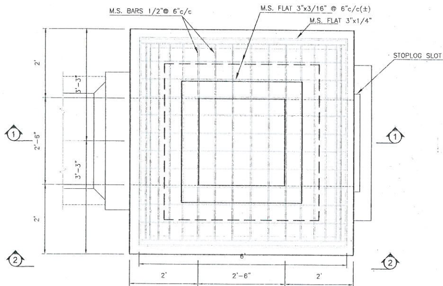
TRASHRACK PLAN INLET STRUCTURE AT EL.3000.0
