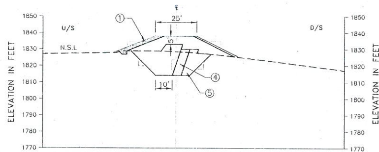
SECTION J-J
