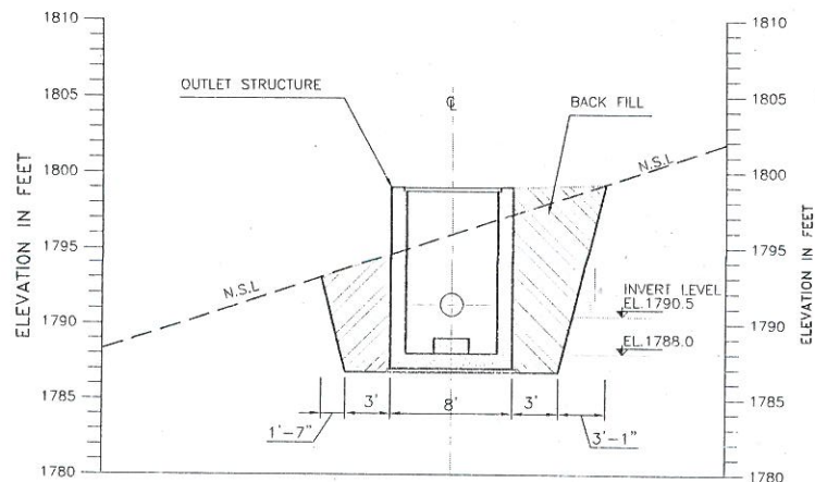
SECTION H-H
