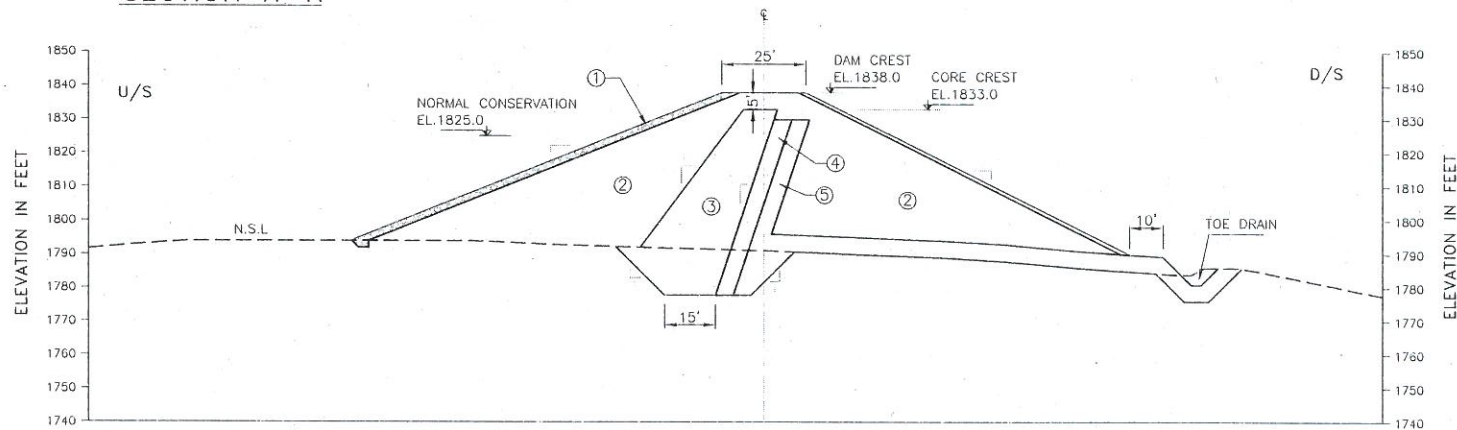
SECTION I-I
