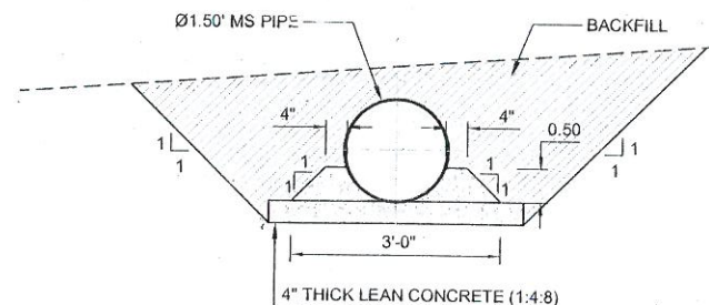
MAIN CANAL PIPE CROSS SECTION
