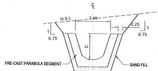
MINOR CANAL TYPICAL CROSS SECTION
