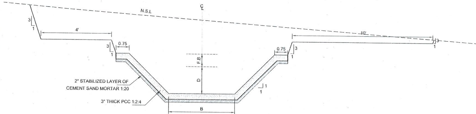
MAIN CANAL TYPICAL CROSS SECTION IN CUT
