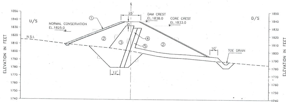
SECTION C-C
