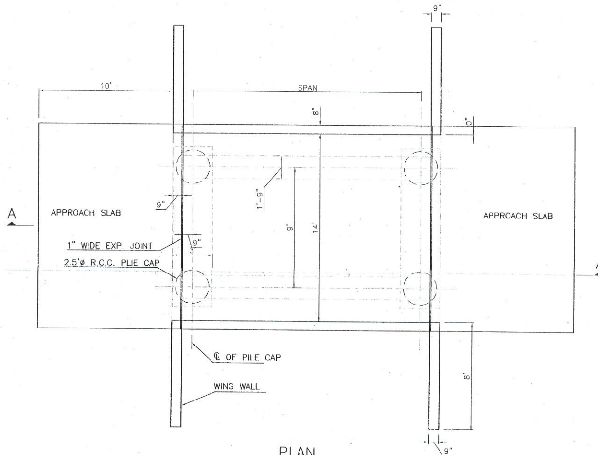
PLAN
