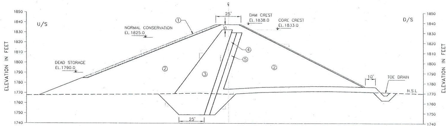
SECTION H-H
