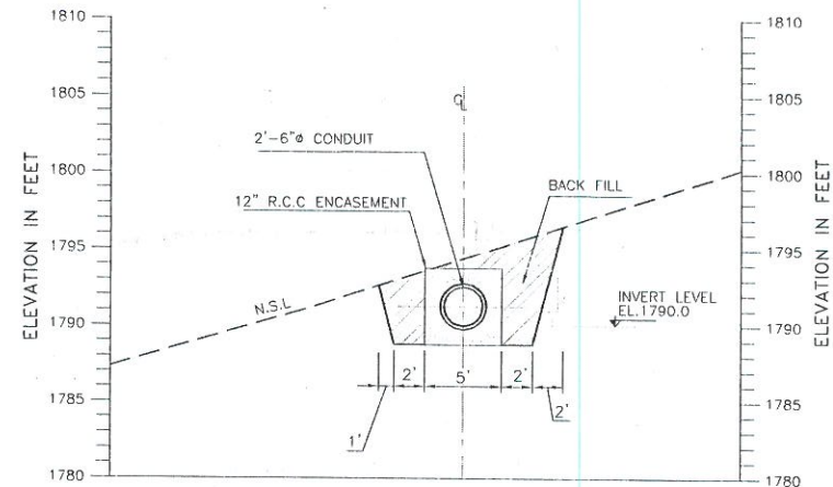
SECTION G-G
