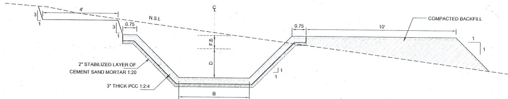
MAIN CANAL TYPICAL CROSS SECTION IN CUT & FILL
