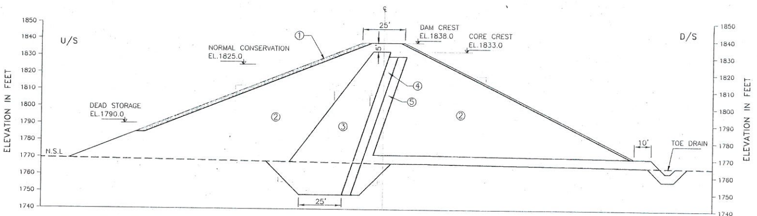
SECTION G-G
