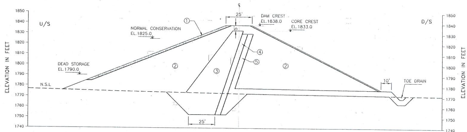
SECTION E-E
