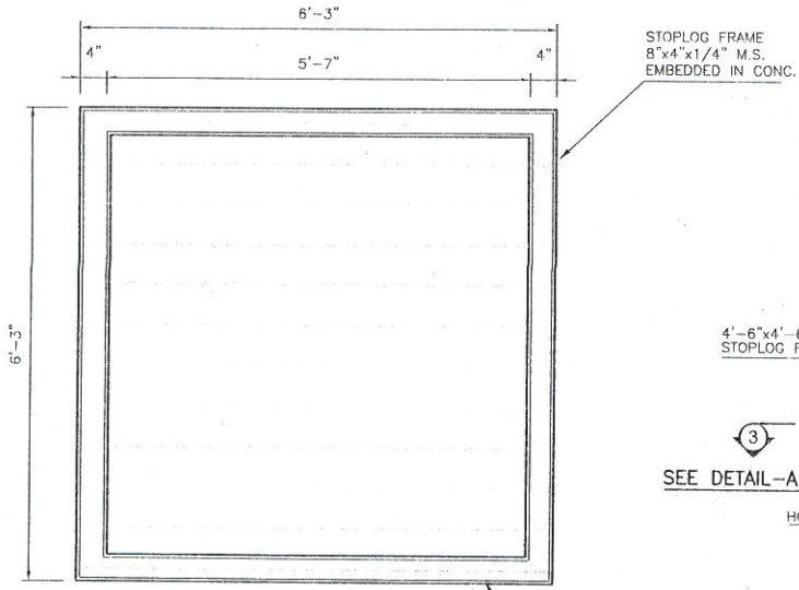
STOPLOG FRAME 3-3 PLAN
