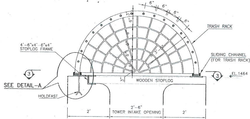
SECTION 1-1
