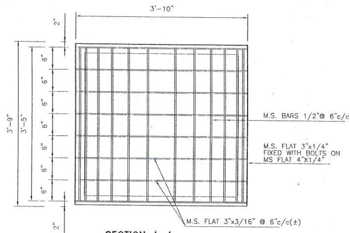
SECTION A-A LOWER TASHRACK ELEVATION
