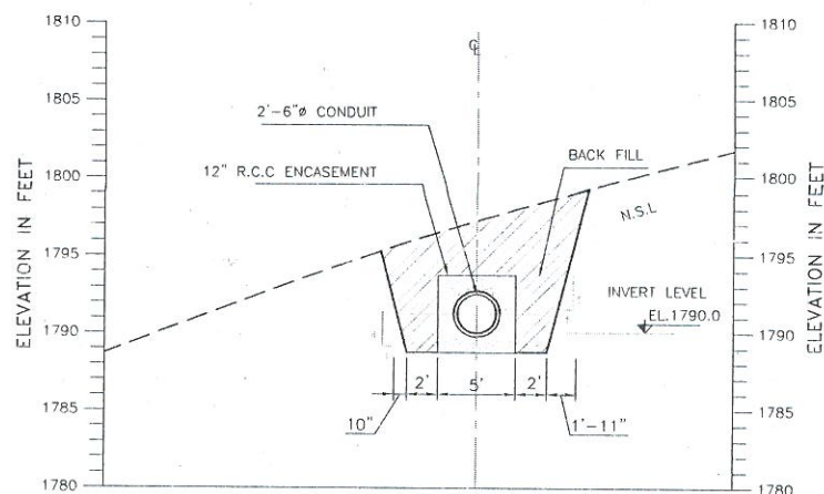
SECTION E-E
