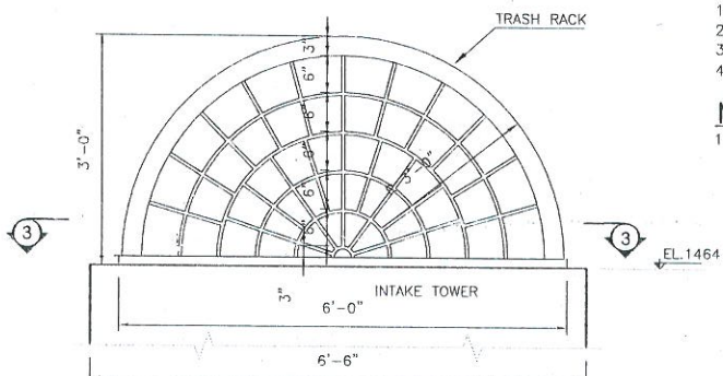
SECTION 2-2 (ELEVATION OF TRASHRACK)
