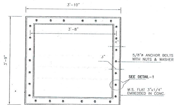
SECTION C-C LOWER TASHRACK FRAME
